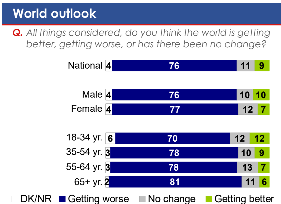
Chart 6: World outlook
