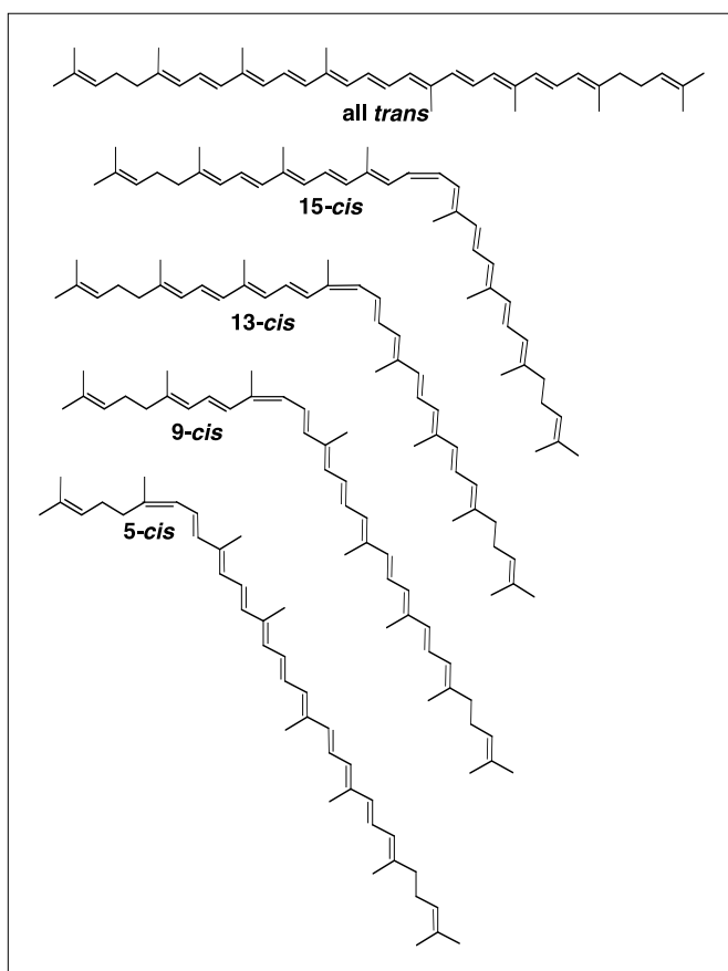
Fig. 1: Structures of trans and cis isomers of lycopene.
