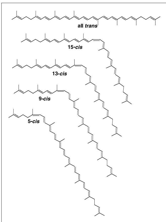
Fig. 1: Structures of trans and cis isomers of lycopene. [Return to text]
