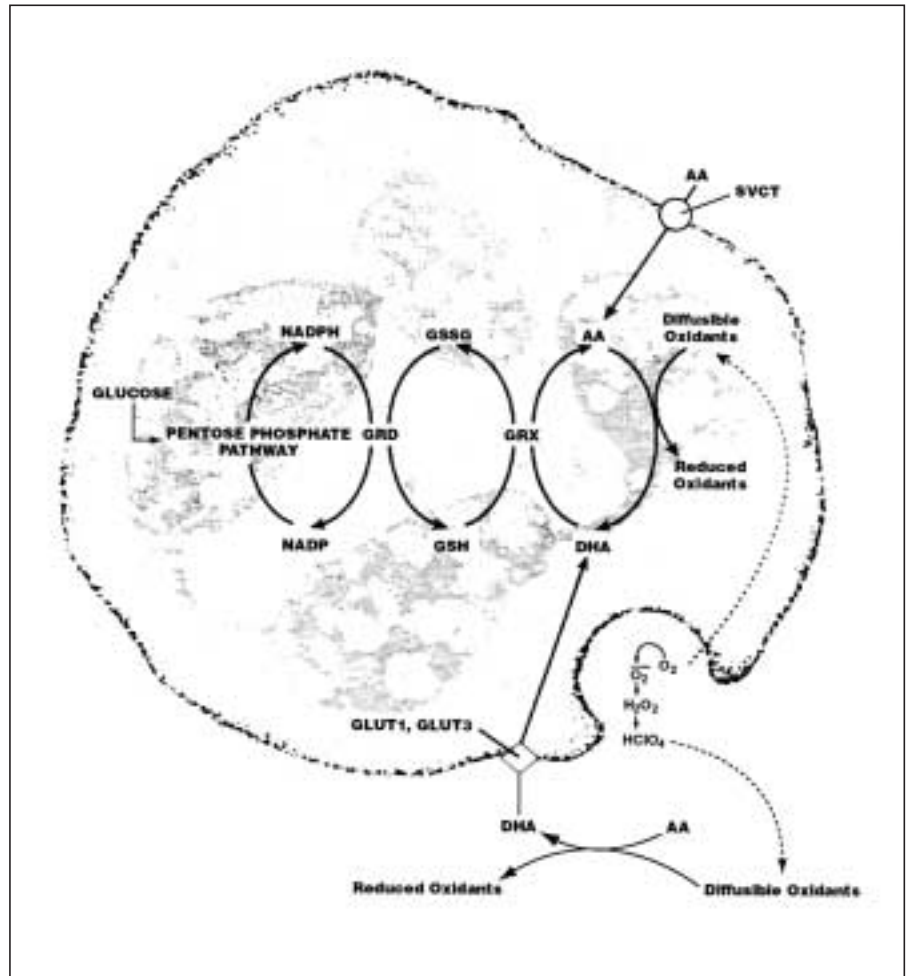
Fig. 1: Ascorbic acid (AA) transport, dehydroascorbic acid (DHA) transport and recycling in human neutrophils. AA, transported by sodium-dependent vitamin C transporters (SVCT), maintains mmol/L concentrations of AA inside neutrophils. Activated neutrophils secrete reactive oxygen species that oxidize extracellular AA to DHA. DHA is rapidly transported into the neutrophil by the glucose transporters GLUT1 and GLUT3 and immediately reduced to AA by glutaredoxin (GRX), producing a 10-fold increase in neutrophil internal AA concentration. Glutathione (GSH), used during DHA reduction, is regenerated from glutathione disulfide (GSSG) by glutathione reductase (GRD) and NADPH. NADPH is a product of glucose metabolism through the pentose phosphate pathway. As NADPH is oxidized to NADP, electrons are transferred to GRD so it can reduce GSSG to GSH. Modified and reproduced with permission of the Journal of Nutritional Biochemistry 1998;9:120, 7 Elsevier Sciences Inc.
