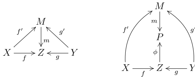
Figure 1: Jointly extremally epimorphic and jointly strongly epimorphic pairs
