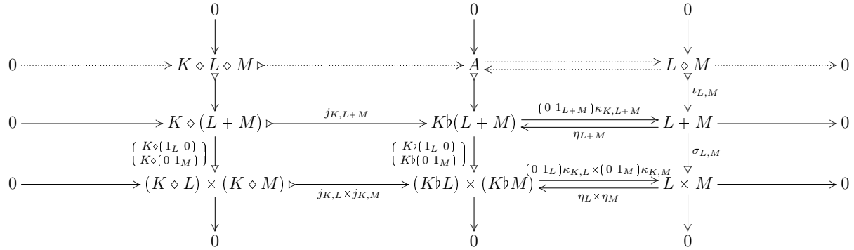
Figure 2: An alternative computation of K \diamond L \diamond M
