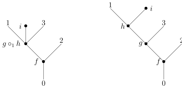
(b) The morphism FU\epsilon_O sends the operation in Figure 1(a) to the O -tree obtained by applying \epsilon_O to the vertex labels.
