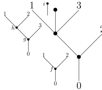
(a) An operation in FUFU(O)_3 .
