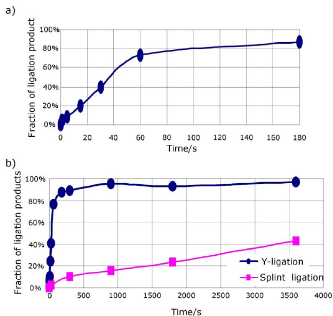
Fig. 3: Time course of ligation reactions. Concentrations were [mRNA] = 0.5 \mu M and [T4 RNA ligase] = 1 U/ \mu l in the enzyme-supplier's buffer with 10% DMSO. At 25 °C.
