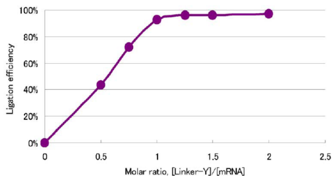
Fig. 4: The dependence of the Y-ligation efficiency on the molar ratio, [Linker-Y]/[mRNA]. Concentration of mRNA was [mRNA] = 0.5 \mu M. The ligation efficiency is defined as the final fraction (at incubation time 3,600s) of the ligation product.
