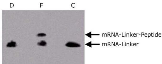
Fig. 5: Virion formation of mRNA-Linker-Y using the Y-ligation. Lane C: control, mRNA-Linker-Y without translation. Lane F: translation product. Lane D: digested translation product by proteinase K.
