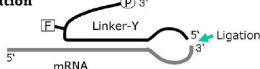
Fig. 1: Scheme of ligation methods of puromycin-linker to mRNA. P and F denote Puromycin and FITC, respectively. The sequence of “Y-ligation loop” is d(CCC) 5' and r(AAAA) 3'.
