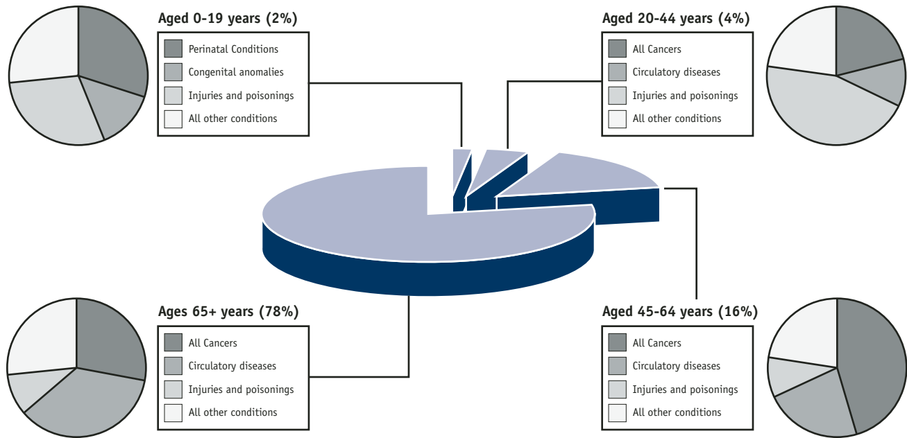
Figure 3.10 Mortality by select causes and age groups, Canada, 2004
