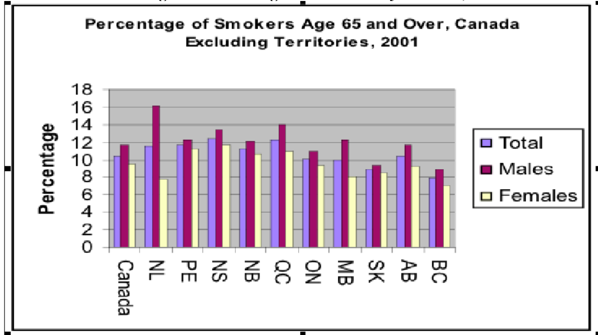
Figure 8.1 Percentage of Smokers Age 65 And Over by Province, 2001
