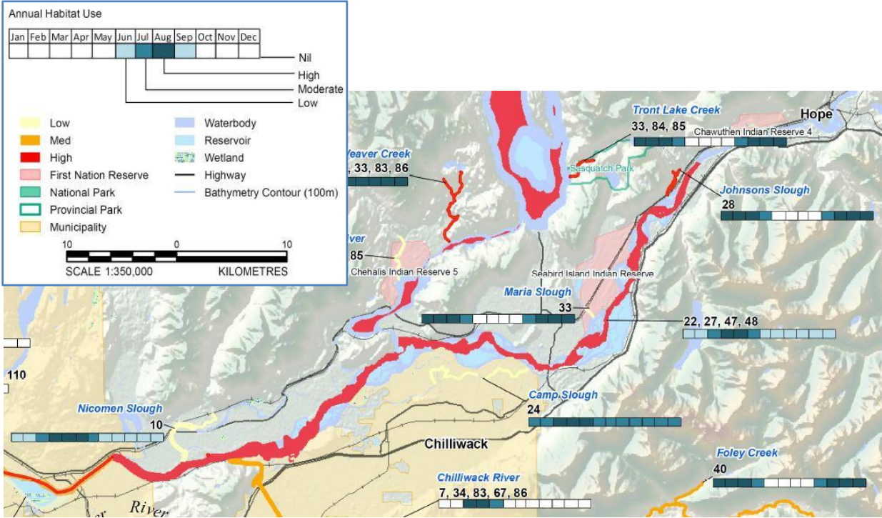
Figure 1. Map 3-B-i: Juvenile Fraser Sockeye Habitat Use in the Lower Fraser River. (Adapted from Cohen Commission Technical Report 12, Map 3-B-i.)
