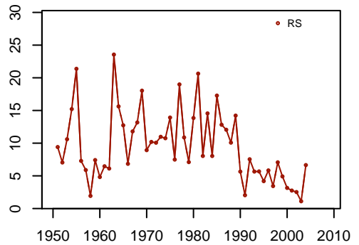
Fraser full total 1950-2004
