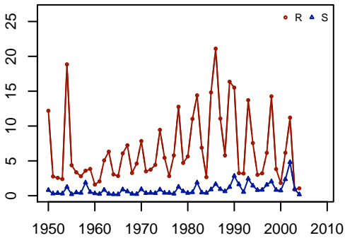
Fraser full 1950-2004 ag
