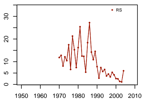
Fraser Summer total 1970-2004
