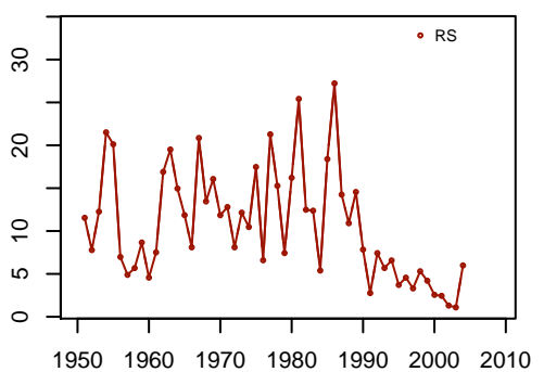
Fraser Summer total 1950-2004
