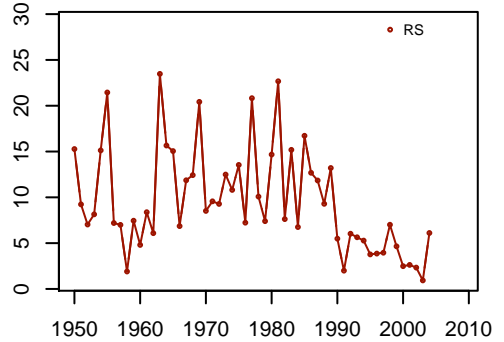
Fraser full 1950-2004 ag
