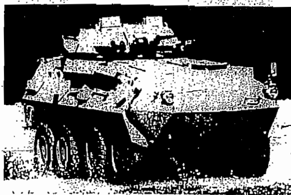
MOWAG Piranha (8 x 8) fitted with two-man turret armed with 25 mm cannon and 7.62 mm machine gun
